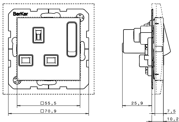
Insert with cover plate Berker S.1, B.3, B.7 Glas
