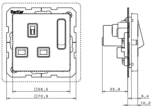
Insert with cover plate Berker Q.1
