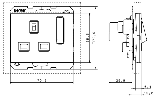
Insert with cover plate Berker K.1/K.5
