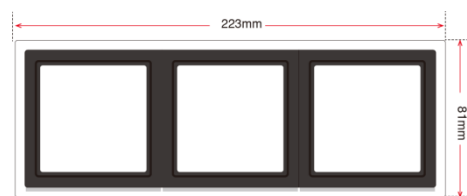
3Gang Frame
